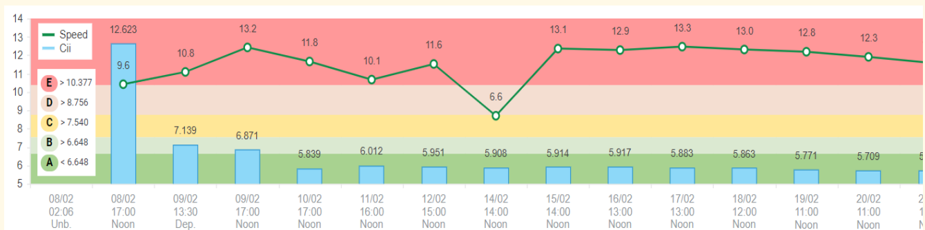
Example of a sea passage rated “A”. As a reminder, the required CII rating for all vessels is “C” as per IMO Regulations
